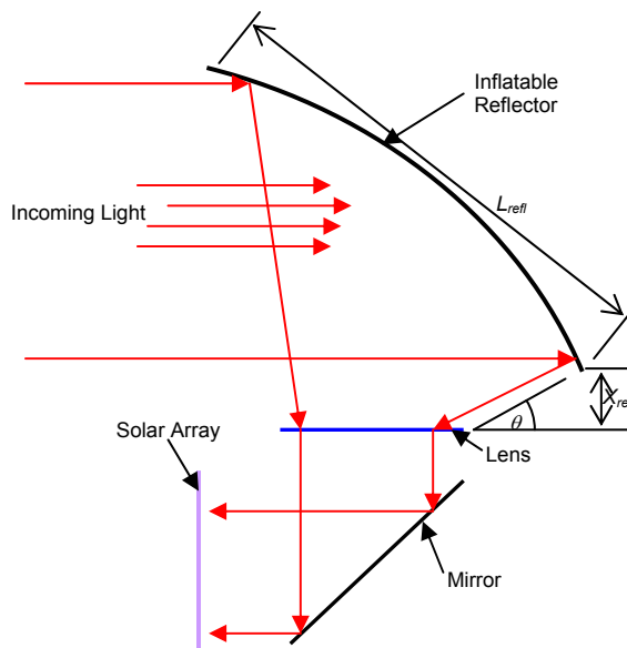
Figure 5: Schematic of the concentrating reflector.
