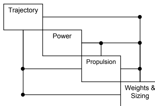
Figure 3: DSM for the SEP module design.
