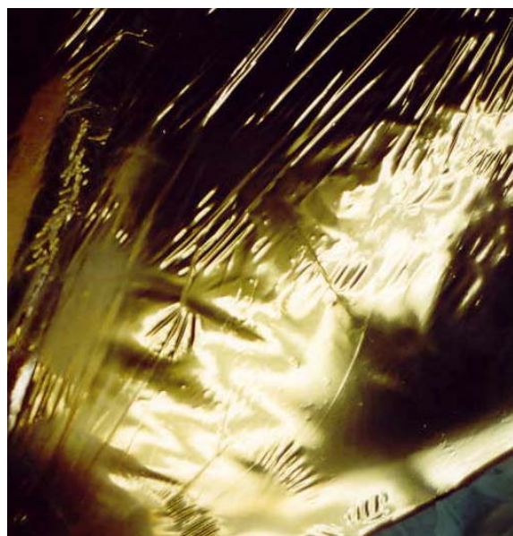
Figure 7: Inflatable reflector surface in mid-heating process. Note the wrinkles in some areas where the mylar hasn't been shrunk yet.
